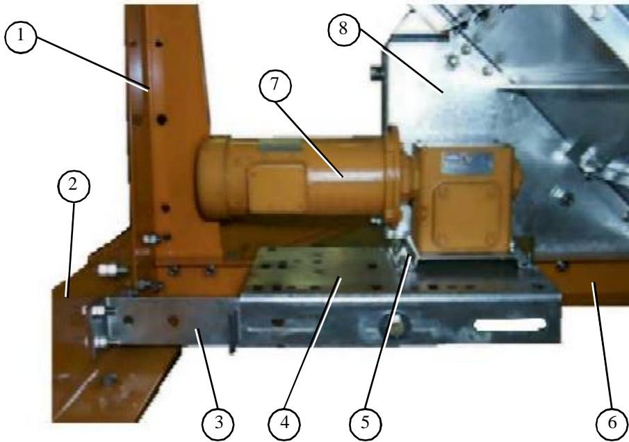
SCR Motor/Reduction drive and motor mount assembly.
